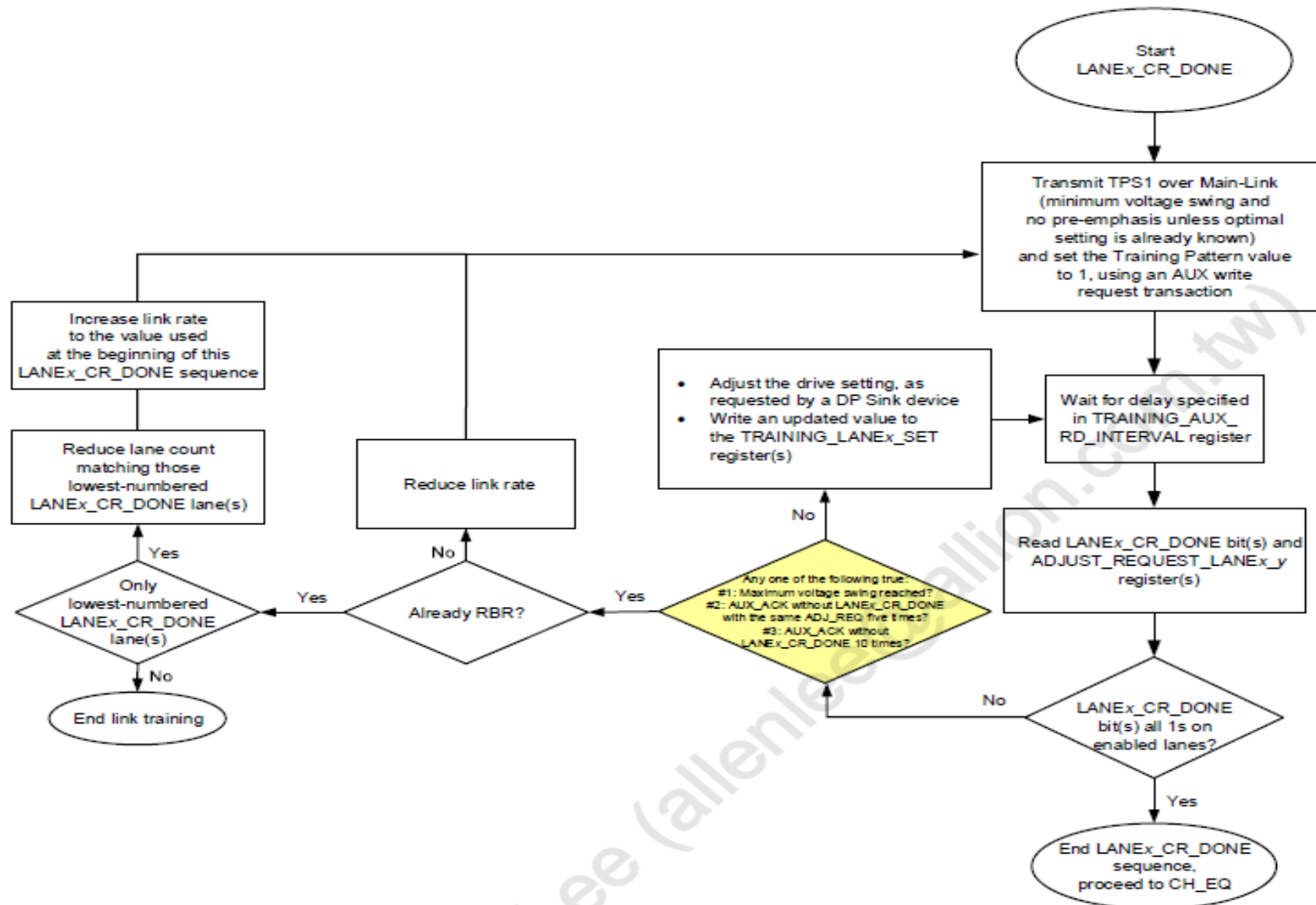
Figure 3-12: Link Training LANEx_CR_Done Sequence
